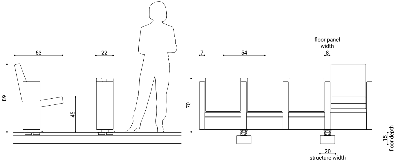
MINIMUM SPACE REQUIREMENT (V9.FLEX)
