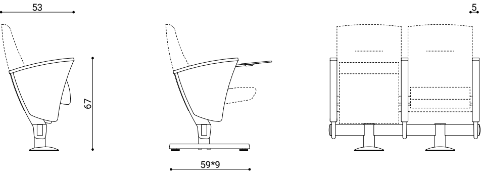
BEAM SIDE / MOBILE LEG
