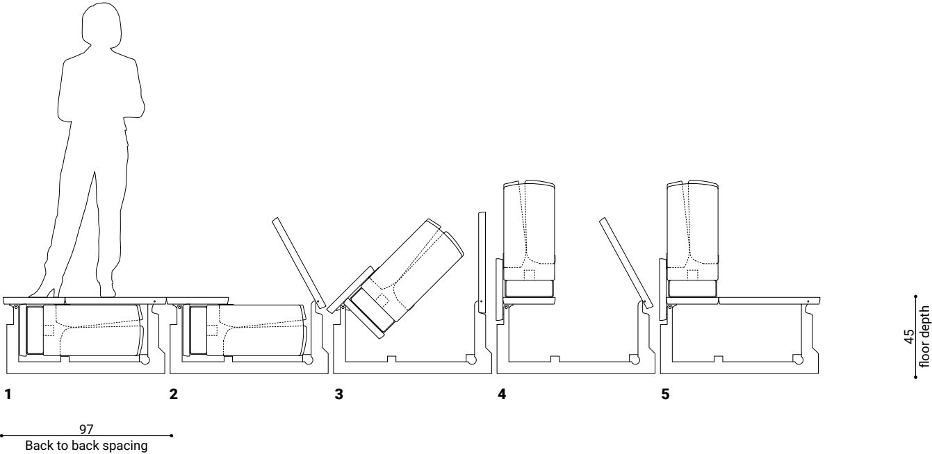
MINIMUM SPACE REQUIREMENT (V9.SYNCRON)
