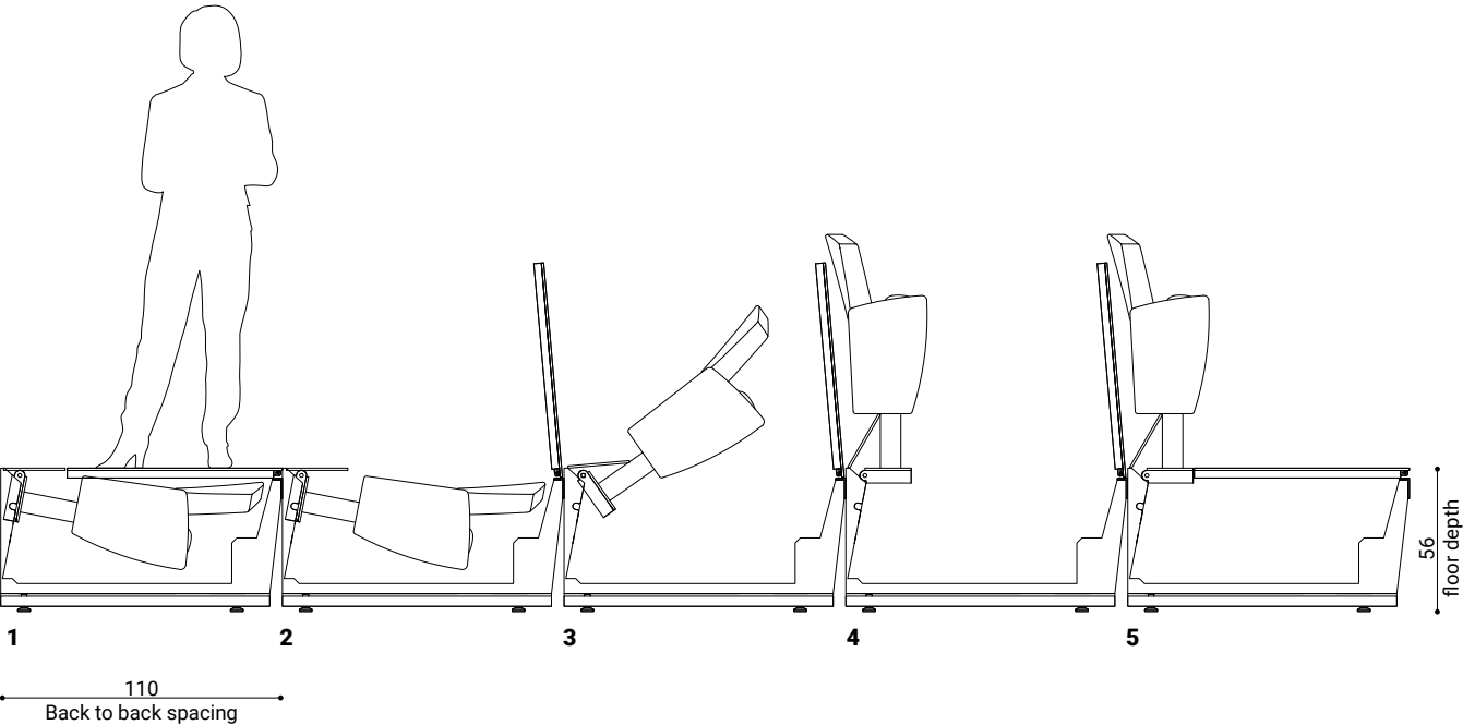
MINIMUM SPACE REQUIREMENT (METROPOLITAN with KURSAAL BEAM side)
