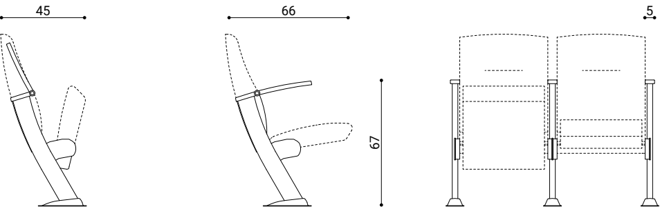
X-ONE WITH FLIP-UP ARMREST SIDE
